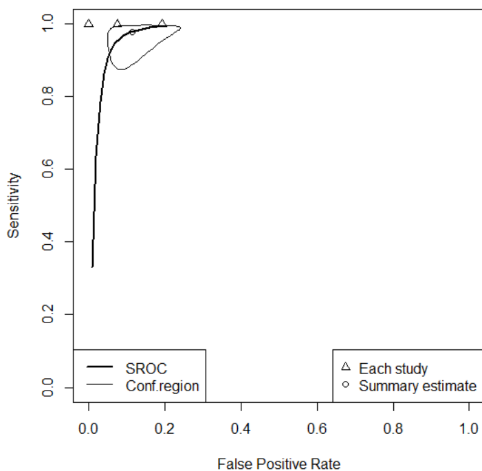
SROC (bivariate model)
